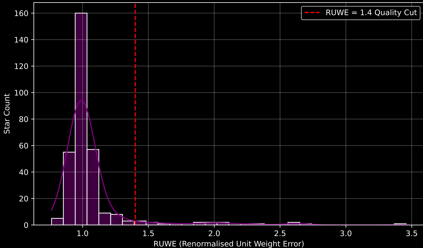
GAPOGEE DR17 Field [M71_MGA] RUWE Distribution (n= 316)
