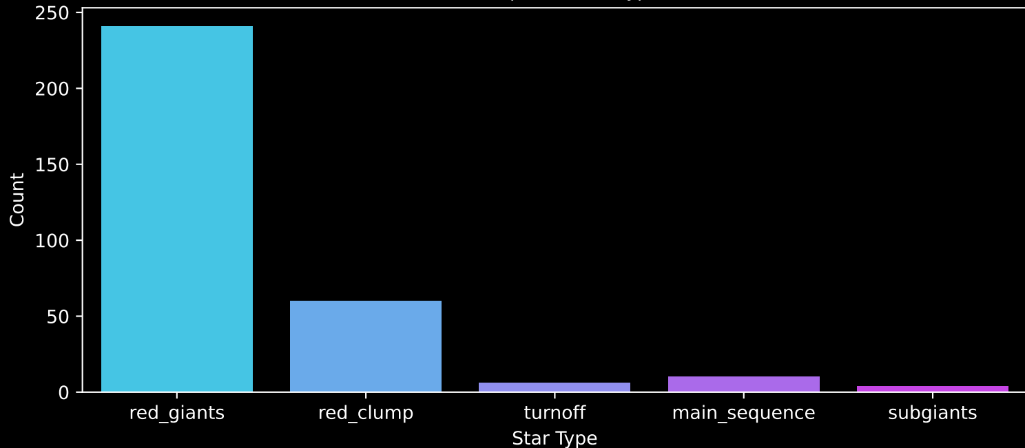
APOGEE DR17 Field: [M71_MGA] Count plot of Star Type
