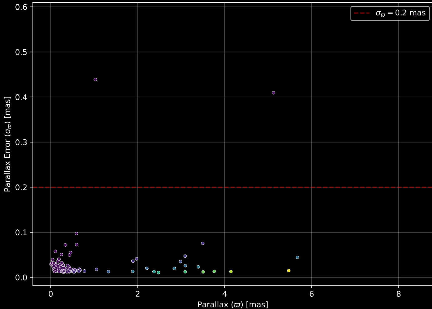
APOGEE DR17 Field: [M71_MGA] Parallax Quality (n= 321)
