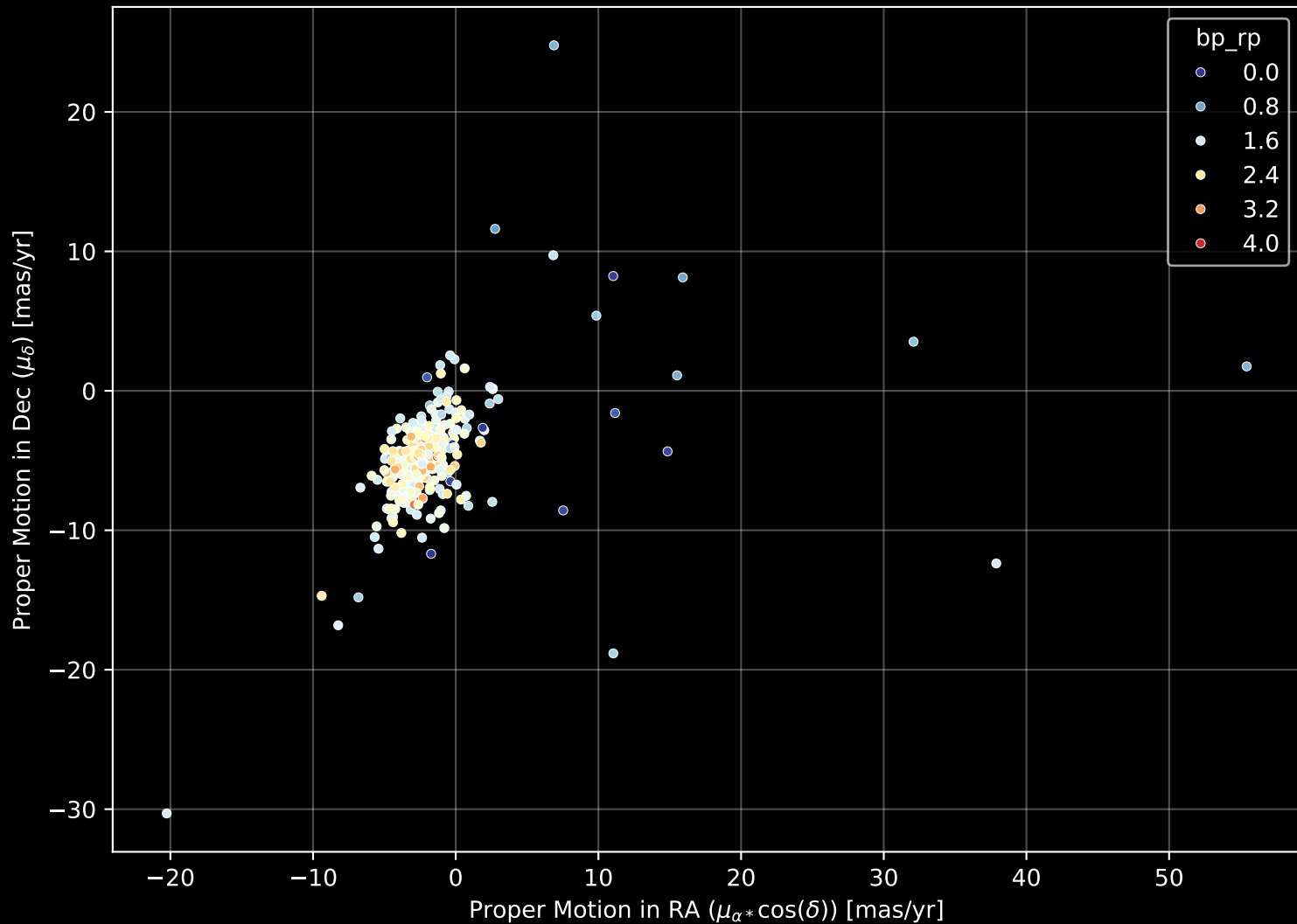
APOGEE DR17 Field: [M71_MGA] Proper Motion Diagram (n= 321)
