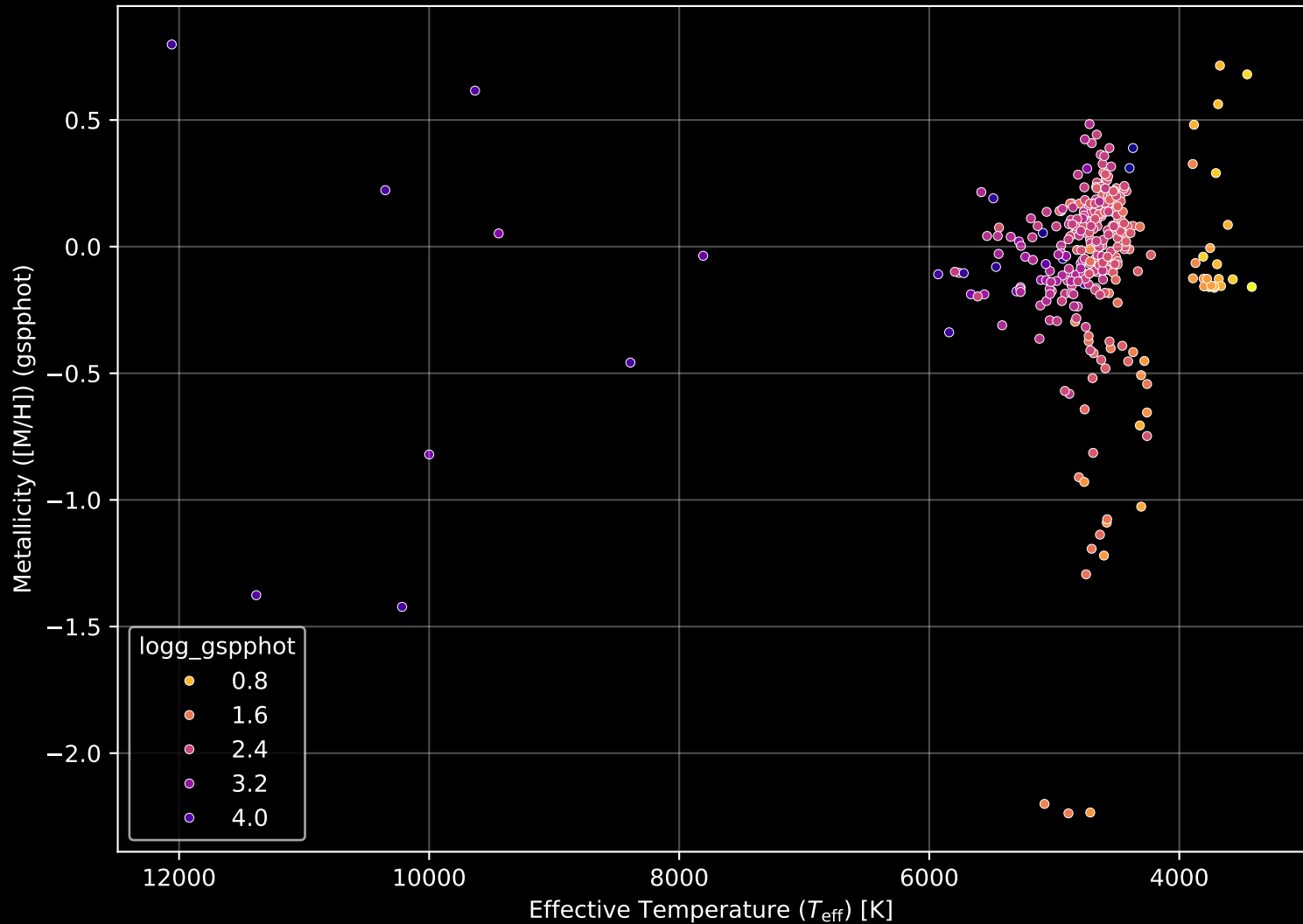
APOGEE DR17 Field: [M71_MGA] Stellar Population Parameters (n= 321)
