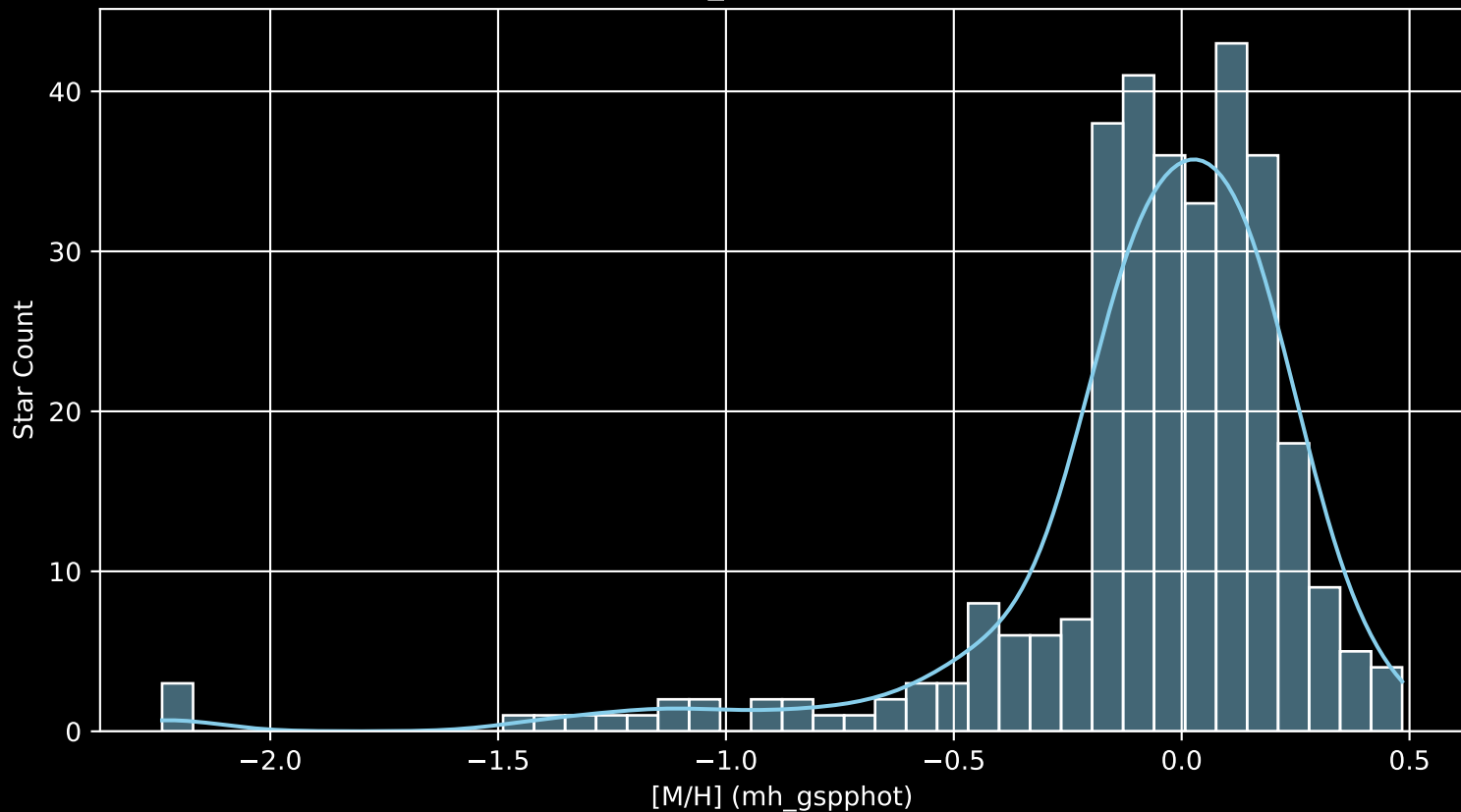
APOGEE DR17 Field: [M71_MGA [M/H] (mh_gspphot) (n= 316)
