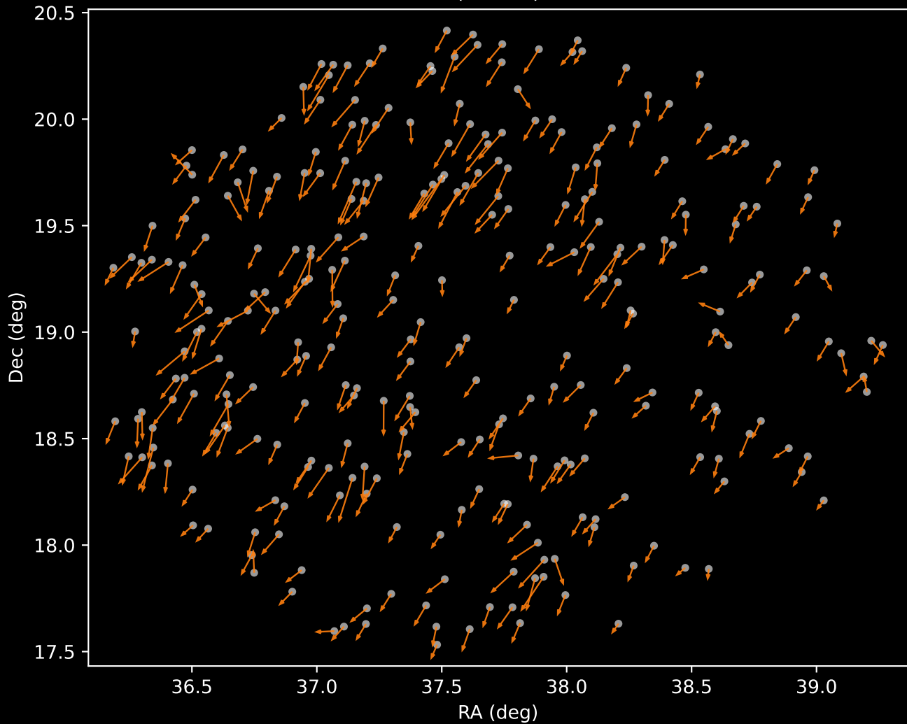
APOGEE DR17 Cluster 2 Proper Motion Vectors (n=291)
